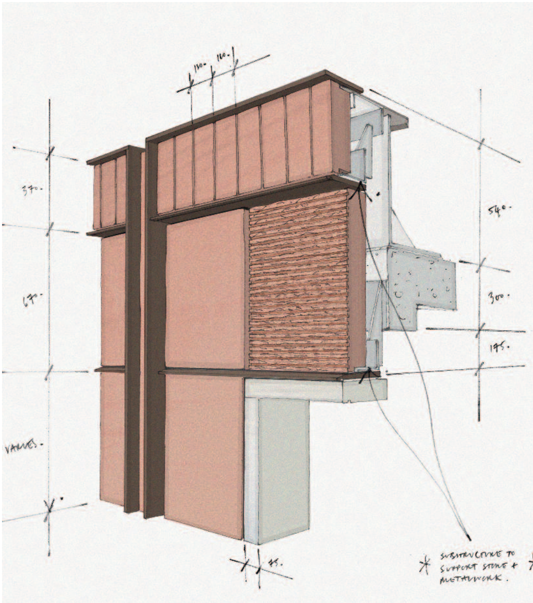
Left Detailed axonometric sketch section through front facade showing stone cladding panels, as well as primary and secondary support structure.
