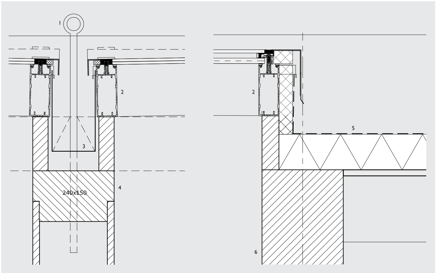
ABOVE Sections through roof showing gutter and parapet conditions: 1 Roof maintenance anchor point 2 aluminium rooflight with UV-barrier and structural glazing 3 EPDM/ aluminium gutter 4 stressed-skin box beam 5 membrane roof 6 cross-laminated timber beam
