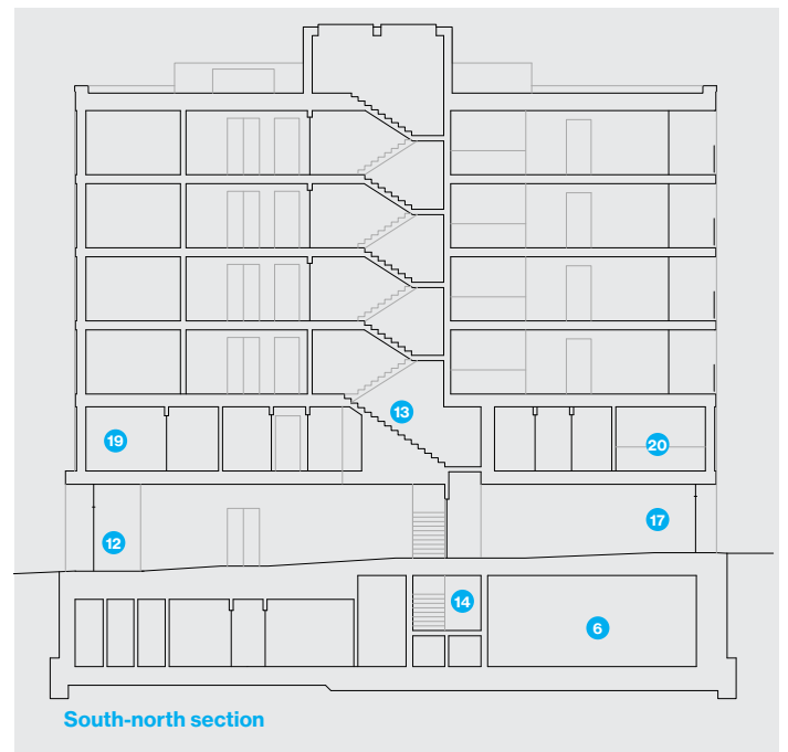
South-north section
