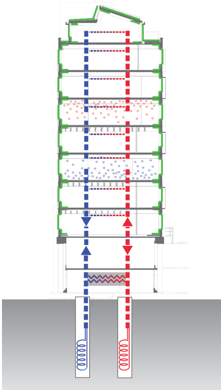
Above Cross-sectional diagram showing aquifer thermal energy store with cool well and warm well.
