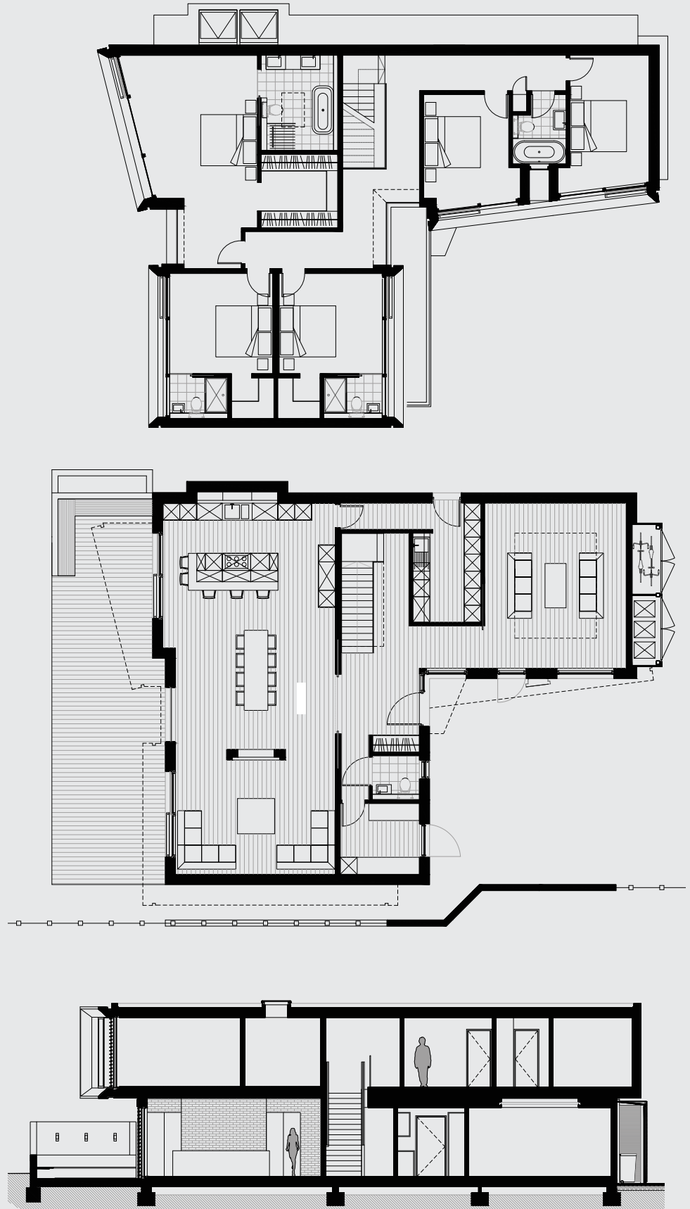
Right Ground- and first-floor plans; section.
